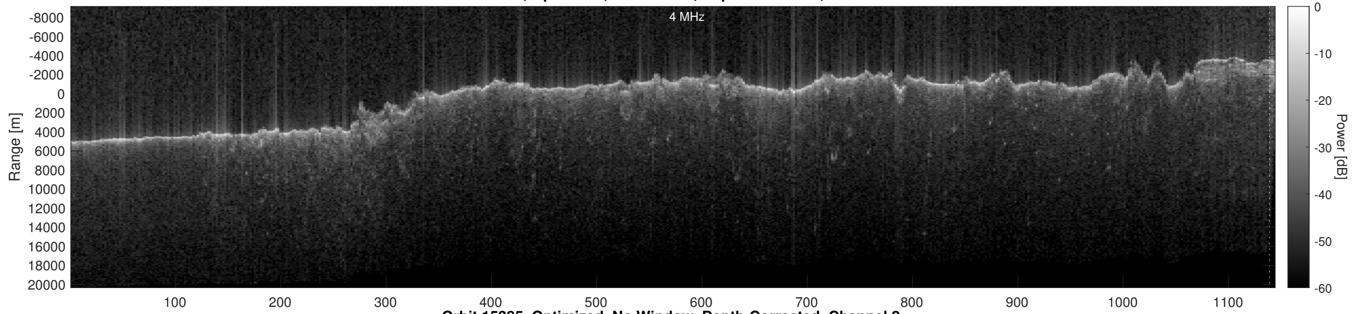
Orbit 15385, Optimized, No Window, Depth-Corrected, Channel 2
