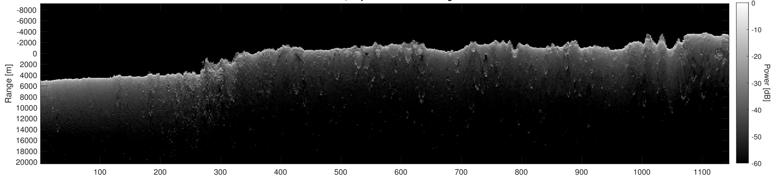
Orbit 15385, Depth-Corrected Cluttergram
