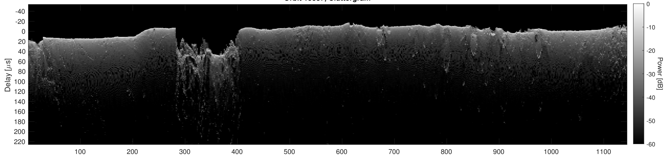
Orbit 15387, Cluttergram
