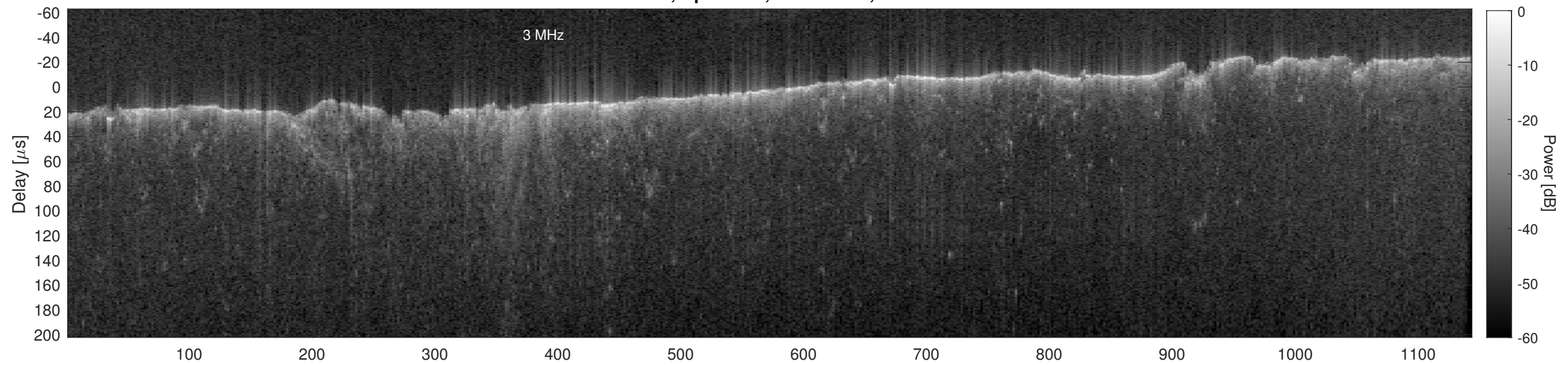
Orbit 15390, Cluttergram
