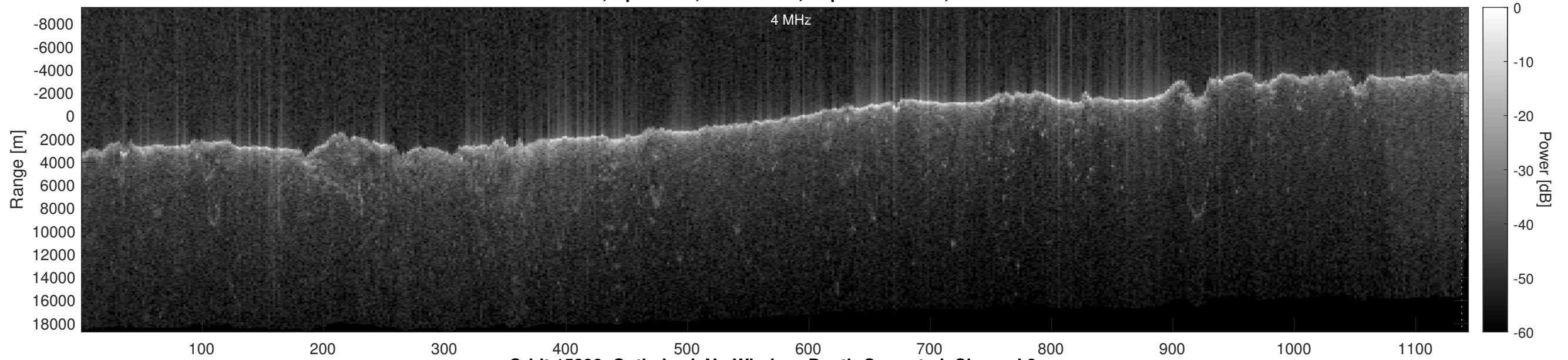
Orbit 15390, Optimized, No Window, Depth-Corrected, Channel 2
