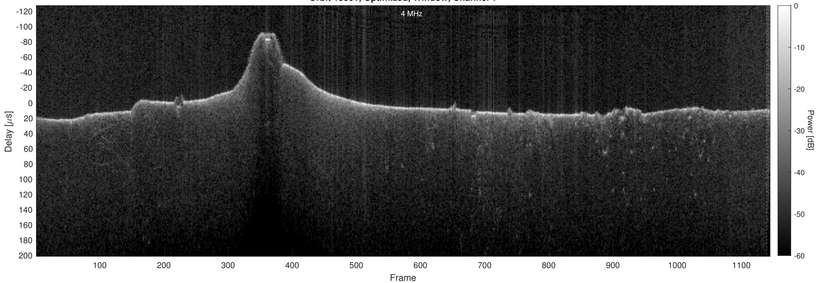
Orbit 15391, Optimized, Window, Channel 2
