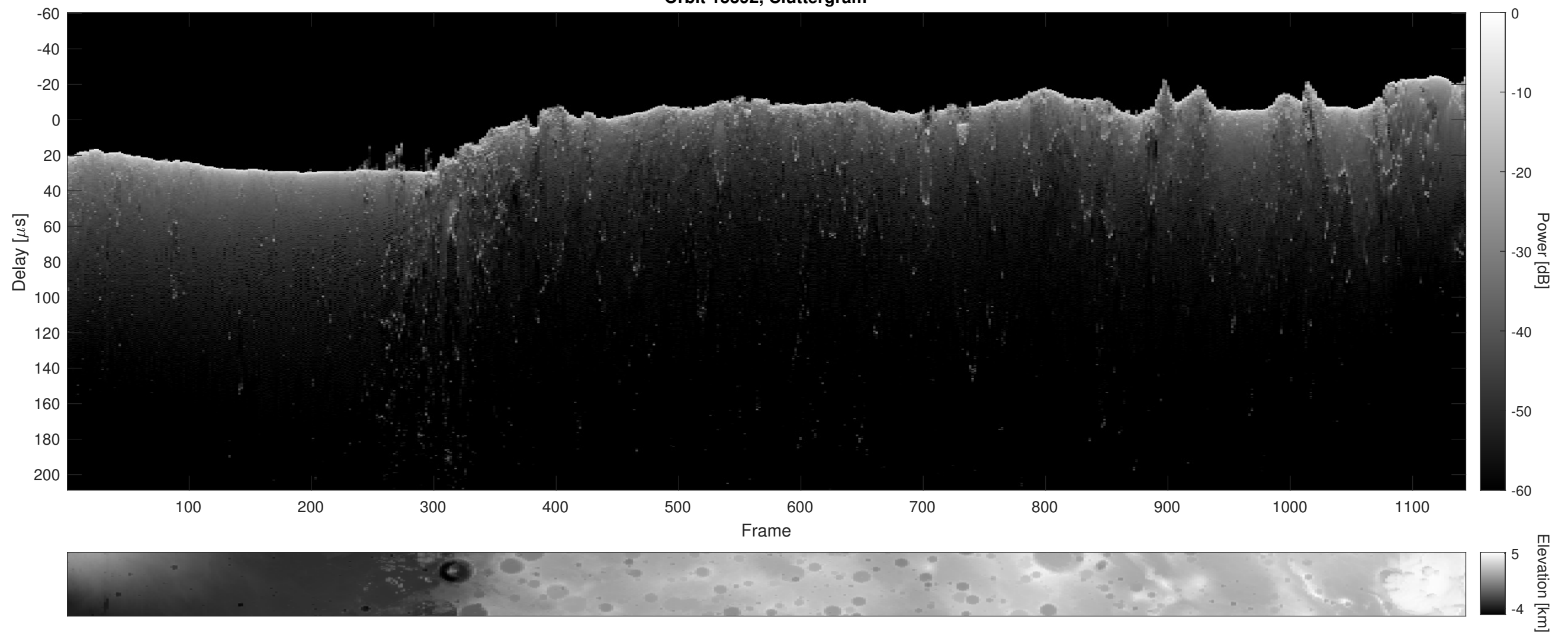
Orbit 15392, Cluttergram
