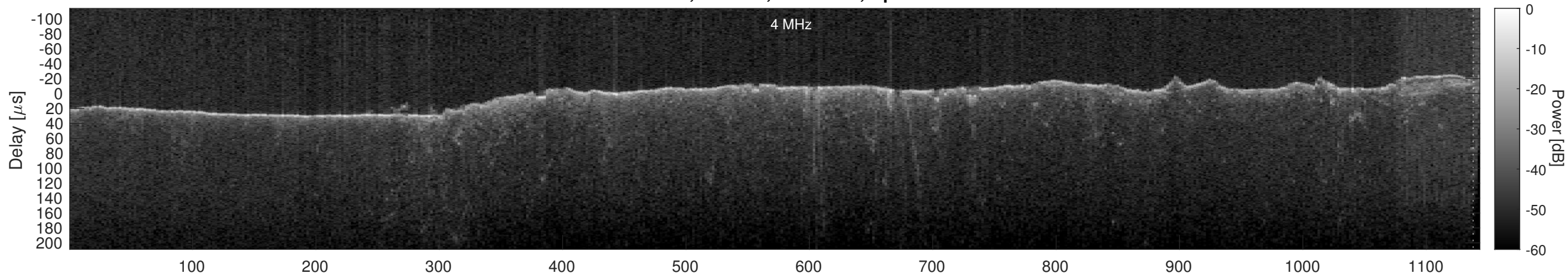
Orbit 15392, Cluttergram
