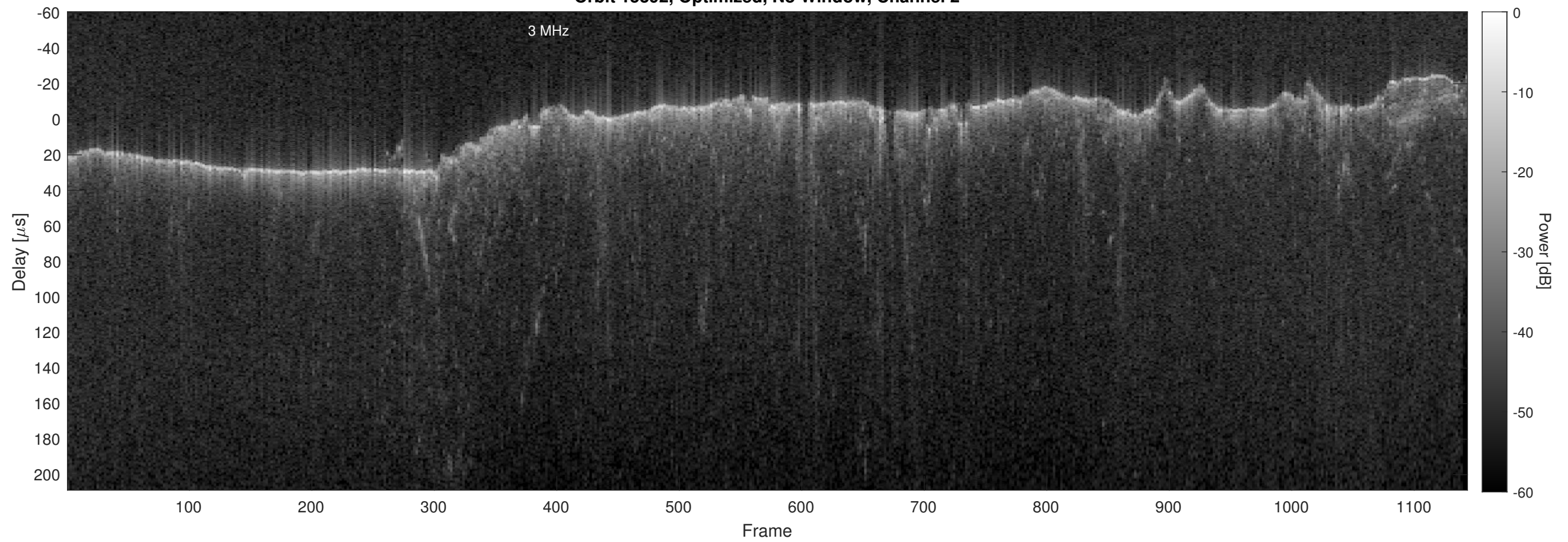
Orbit 15392, Optimized, No Window, Channel 2
