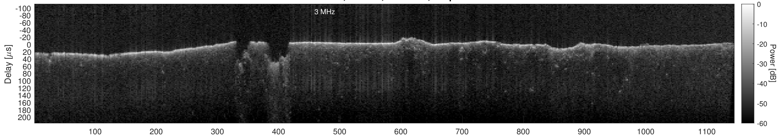
Orbit 15394, Window, Channel 2, Optimized
