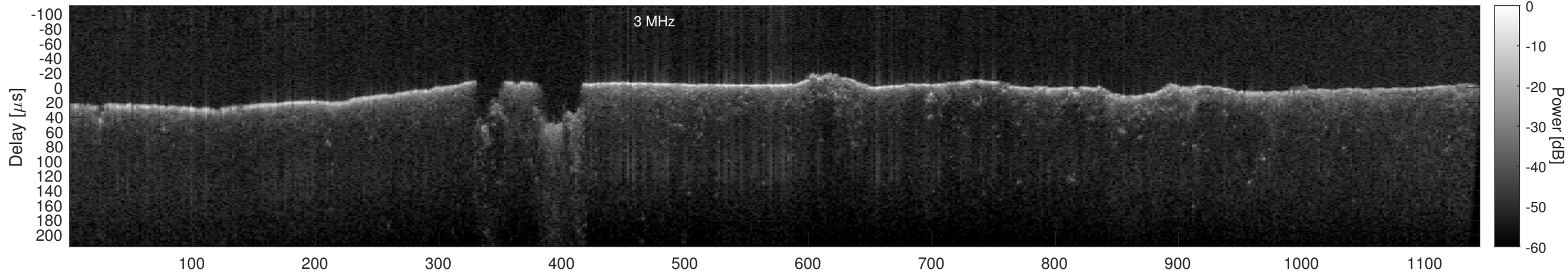
Orbit 15394, Window, Channel 2, Chapman
