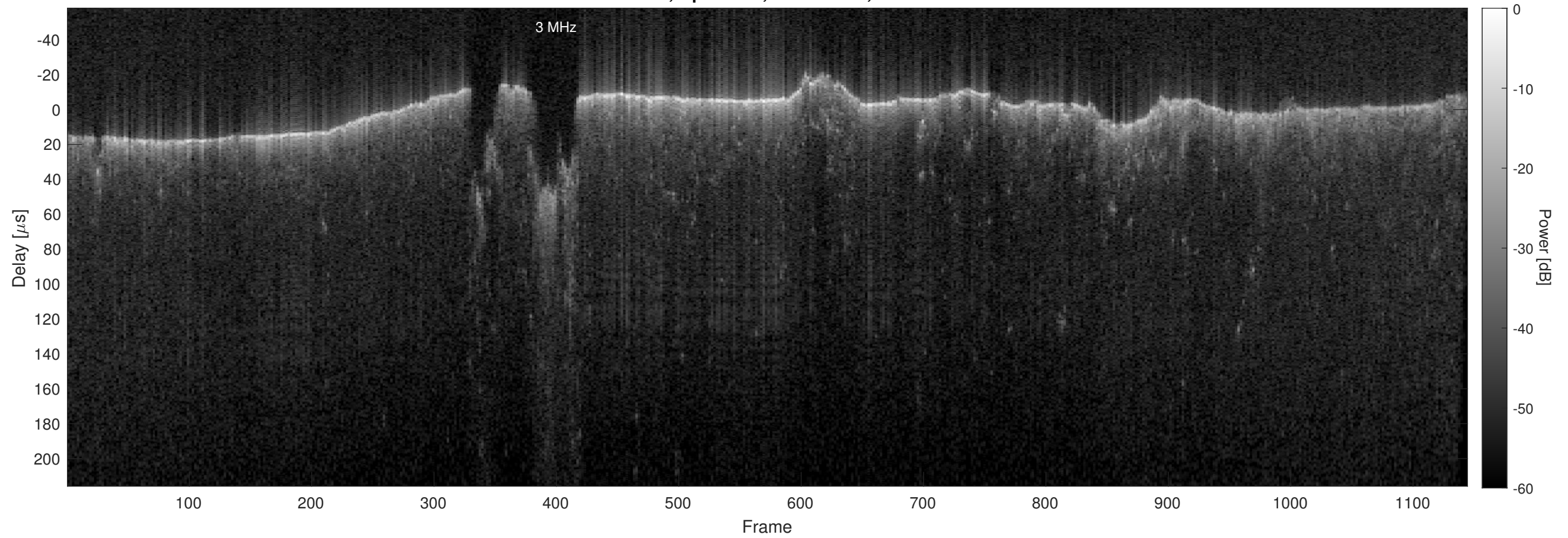
Orbit 15394, Optimized, No Window, Channel 2
