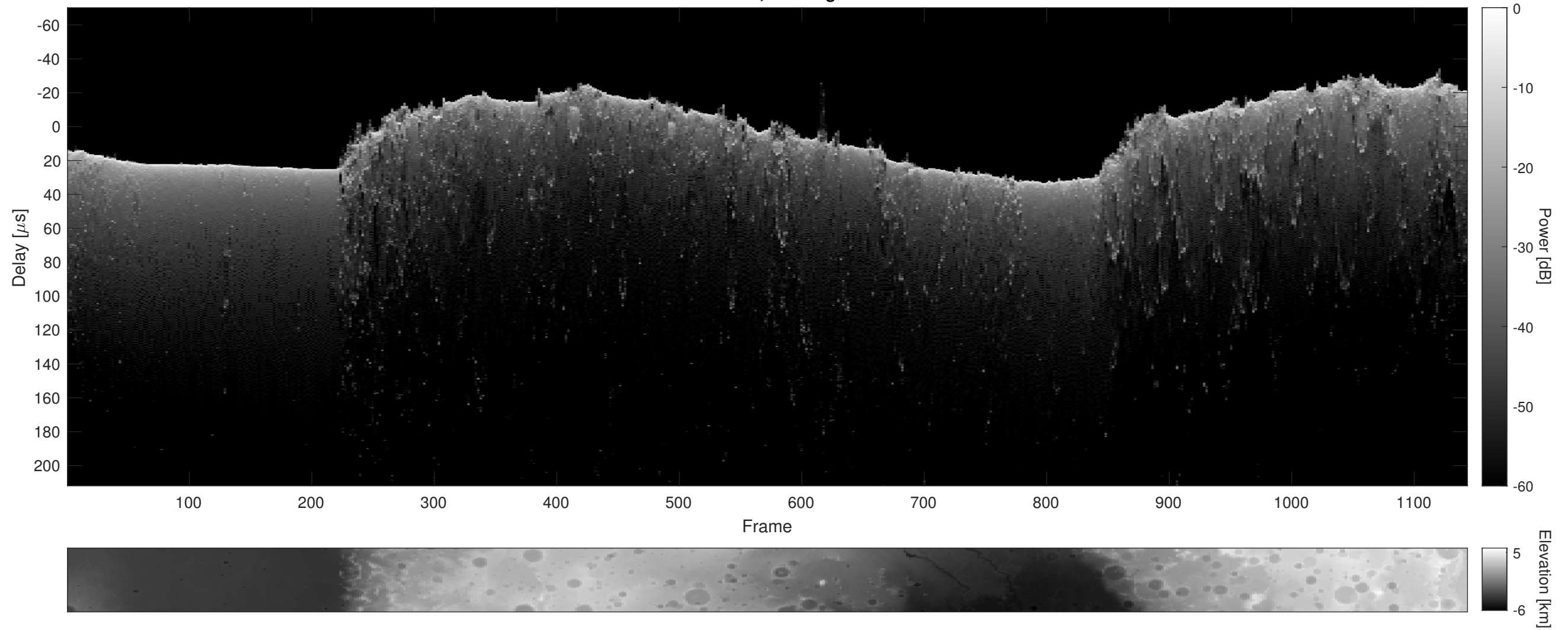
Orbit 15396, Cluttergram
