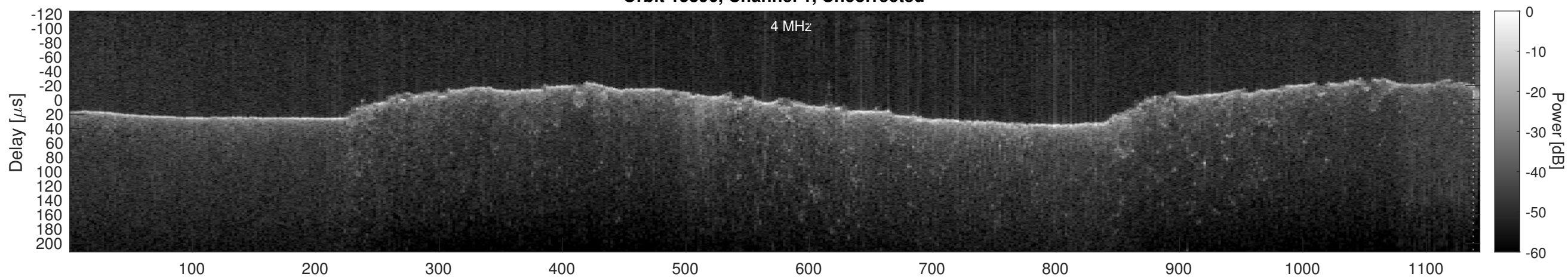
Orbit 15396, Window, Channel 1, Chapman
