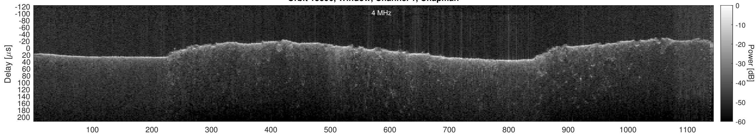
Orbit 15396, Window, Channel 1, Optimized
