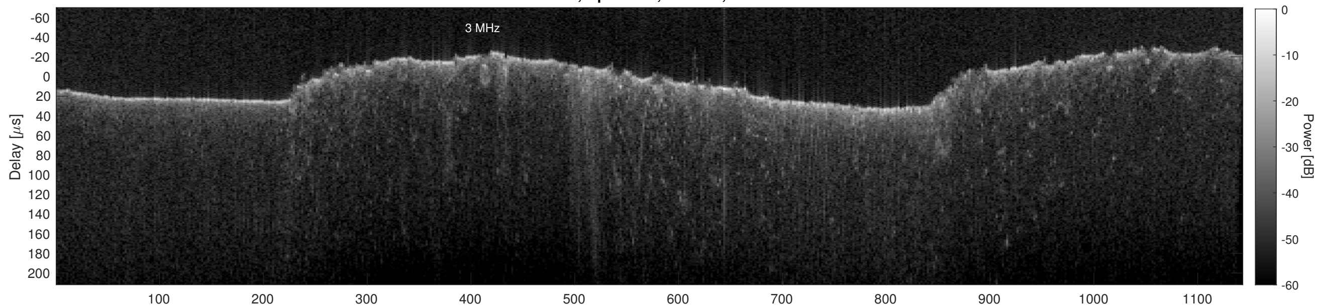
Orbit 15396, Cluttergram
