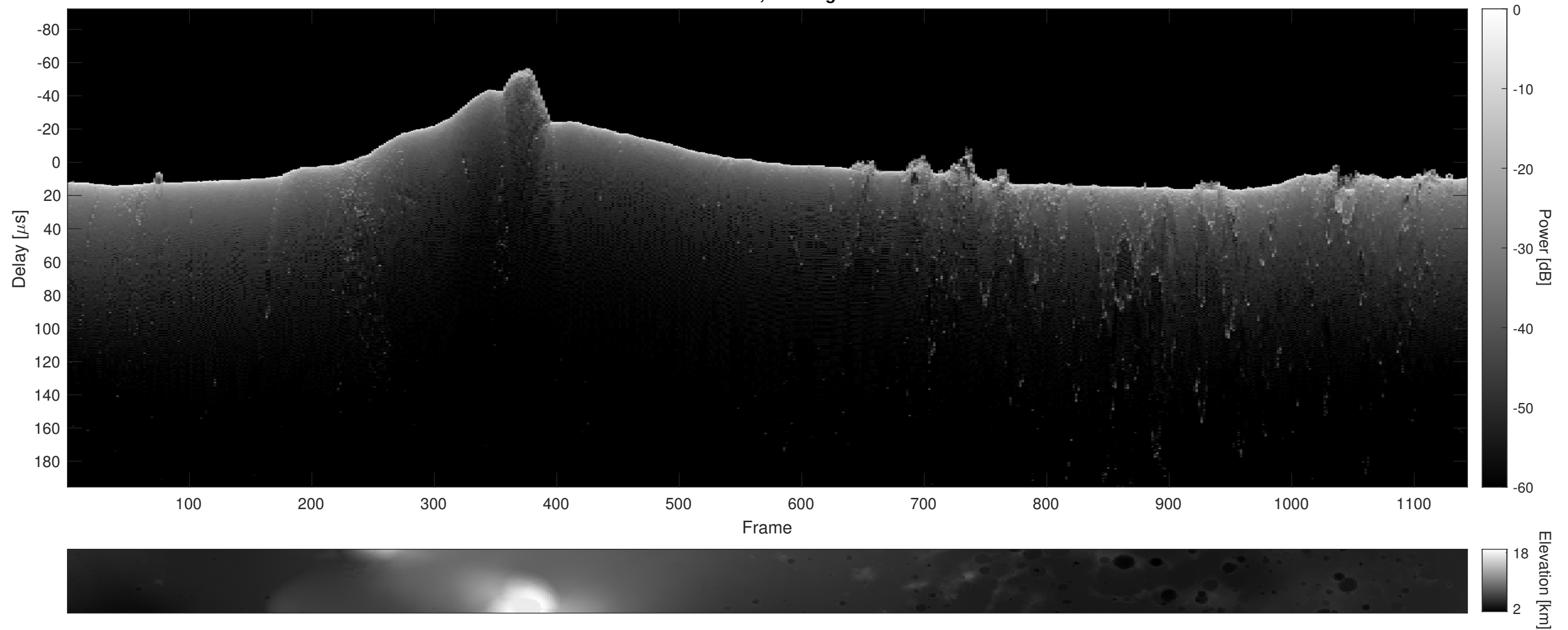
Orbit 15398, Cluttergram
