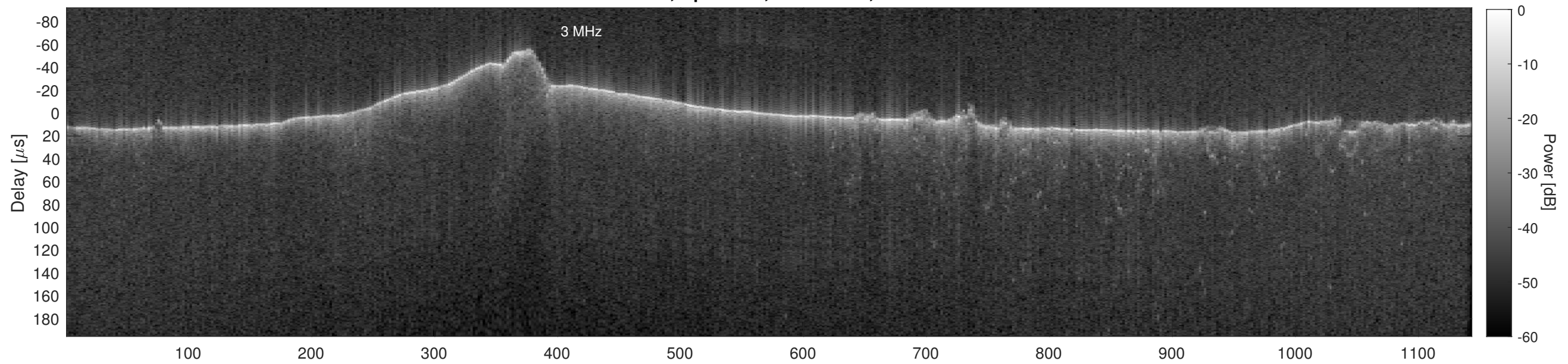
Orbit 15398, Cluttergram
