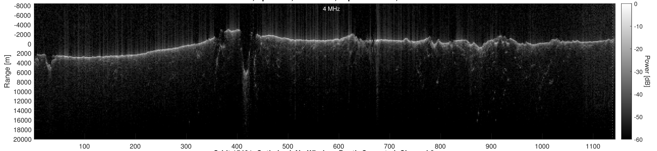
Orbit 15401, Optimized, No Window, Depth-Corrected, Channel 2
