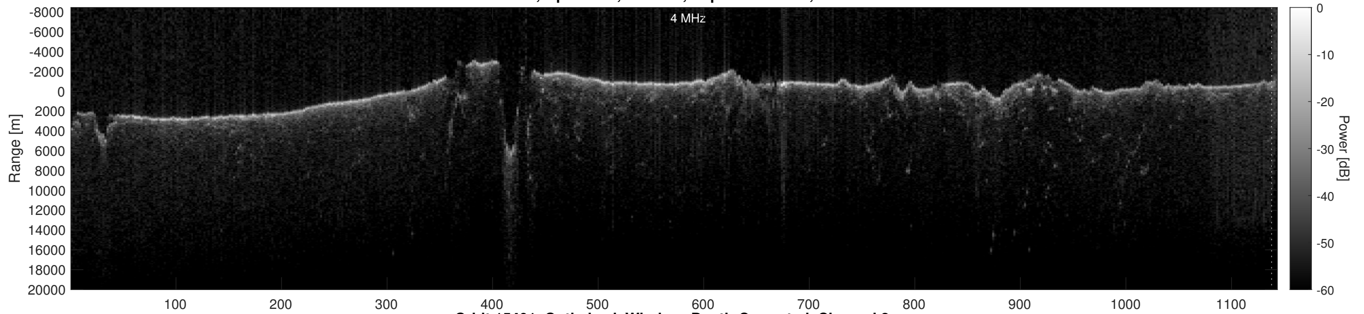
Orbit 15401, Optimized, Window, Depth-Corrected, Channel 2
