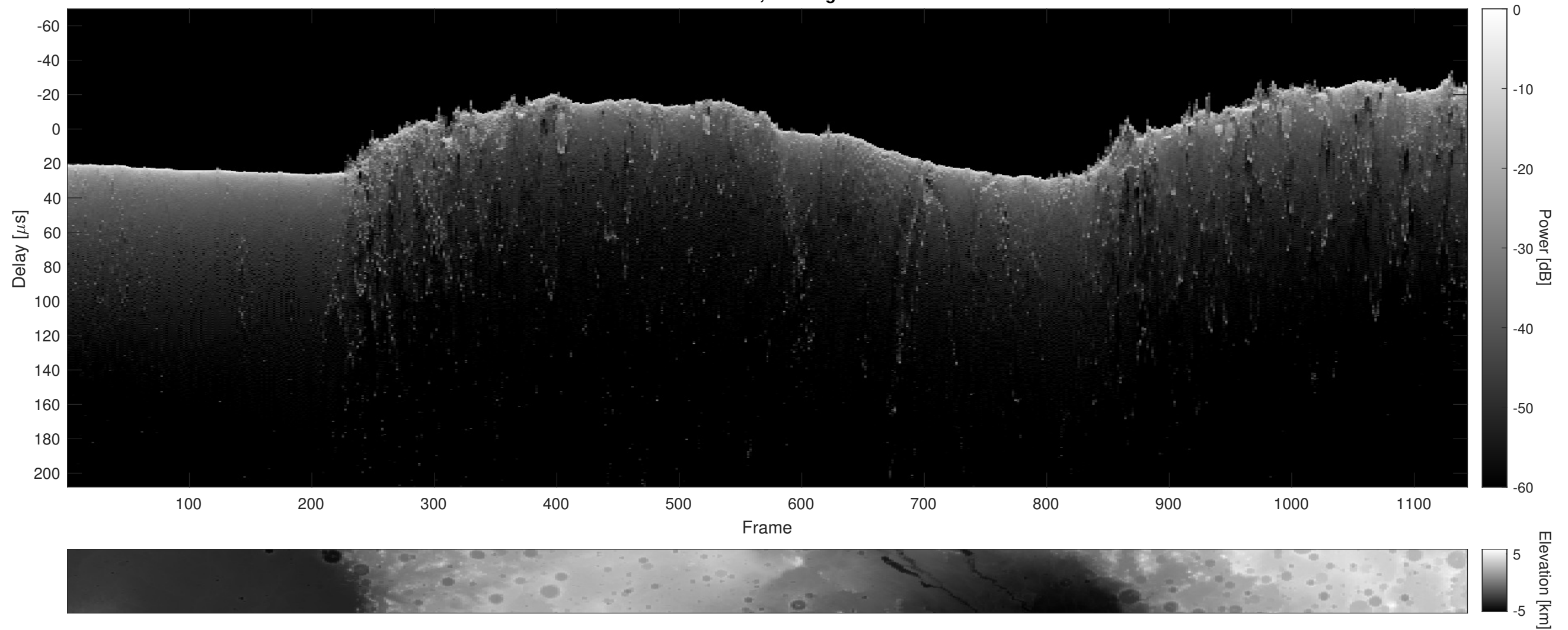
Orbit 15403, Cluttergram
