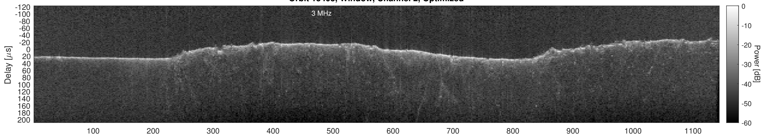
Orbit 15403, Cluttergram
