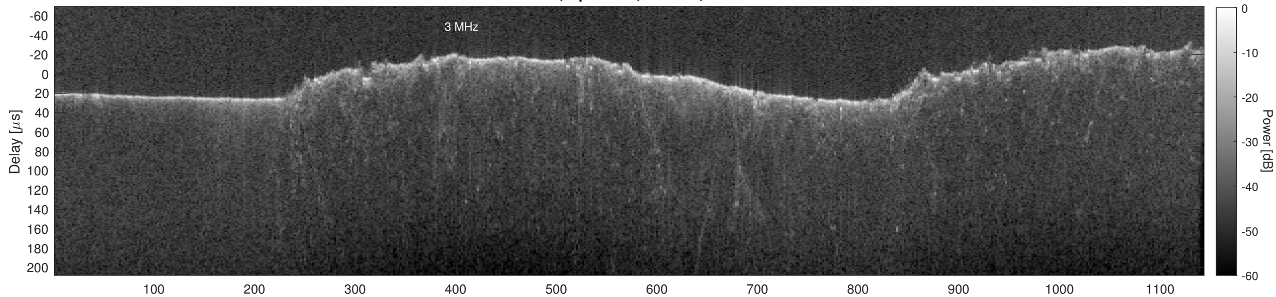
Orbit 15403, Cluttergram
