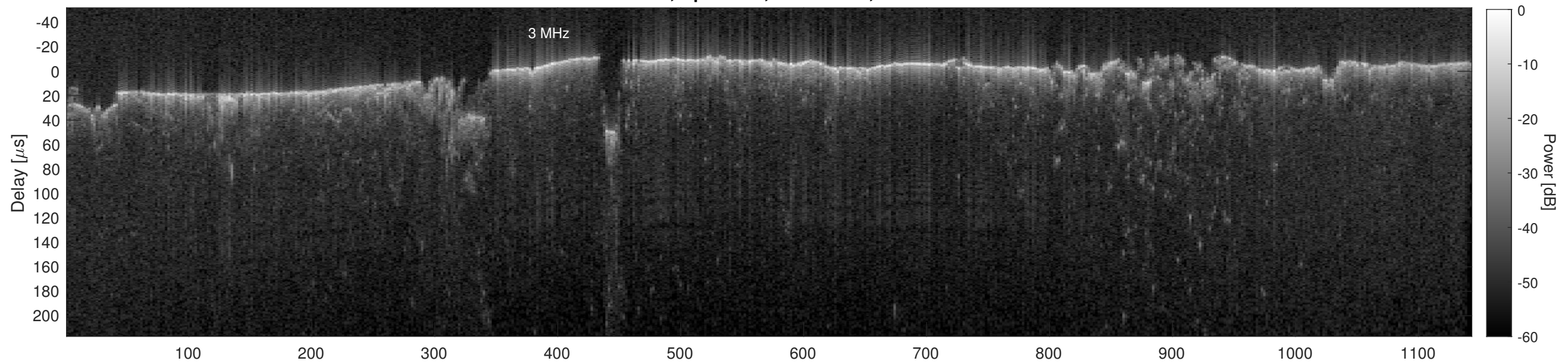
Orbit 15408, Cluttergram
