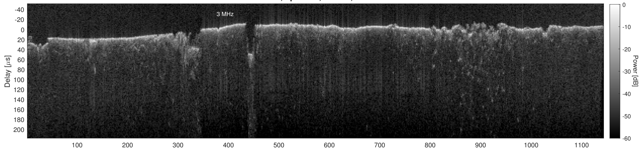
Orbit 15408, Cluttergram
