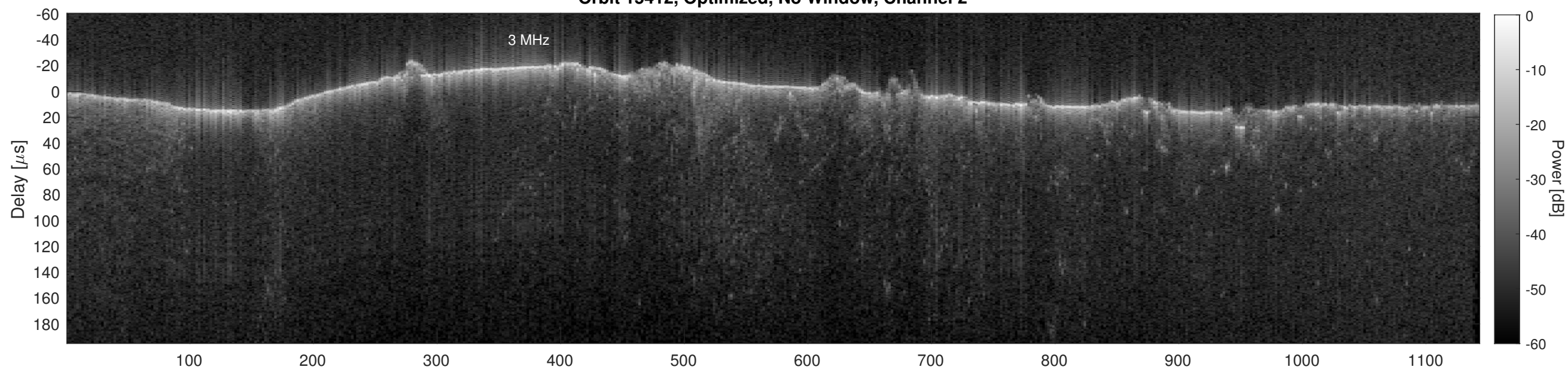
Orbit 15412, Cluttergram
