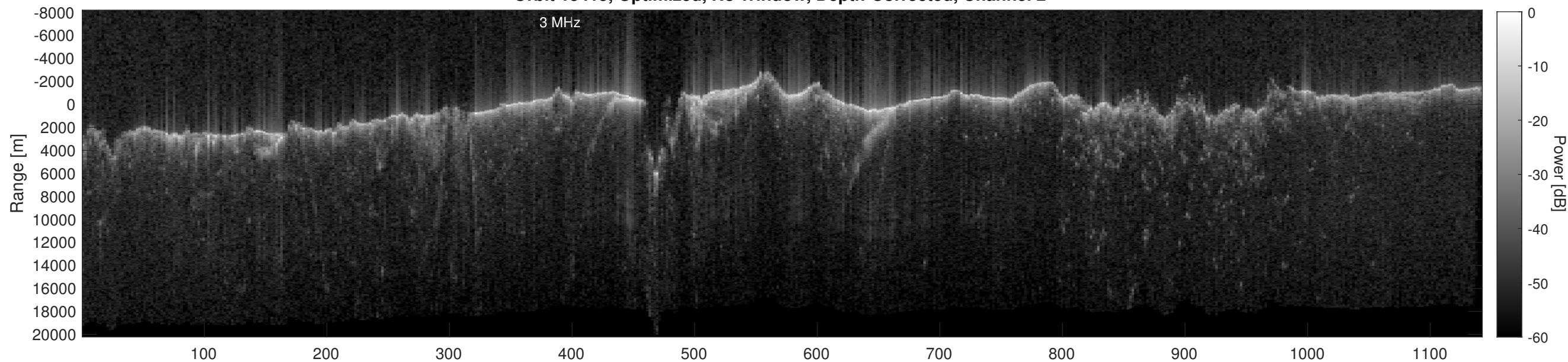
Orbit 15415, Depth-Corrected Cluttergram
