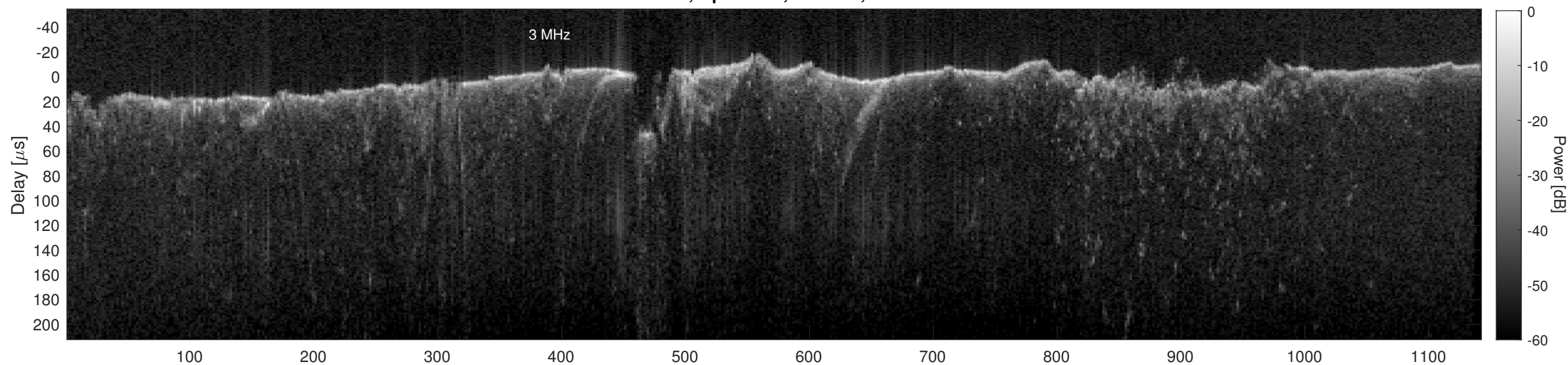
Orbit 15415, Cluttergram
