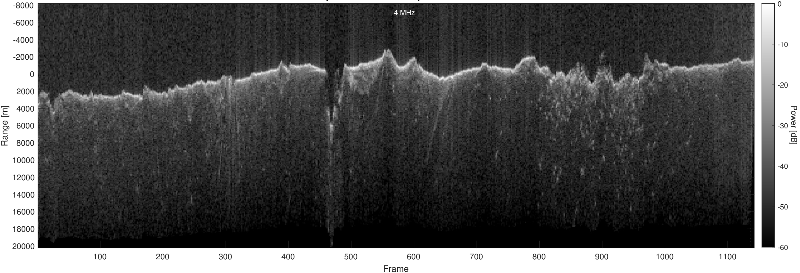
Orbit 15415, Optimized, Window, Depth-Corrected, Channel 2
