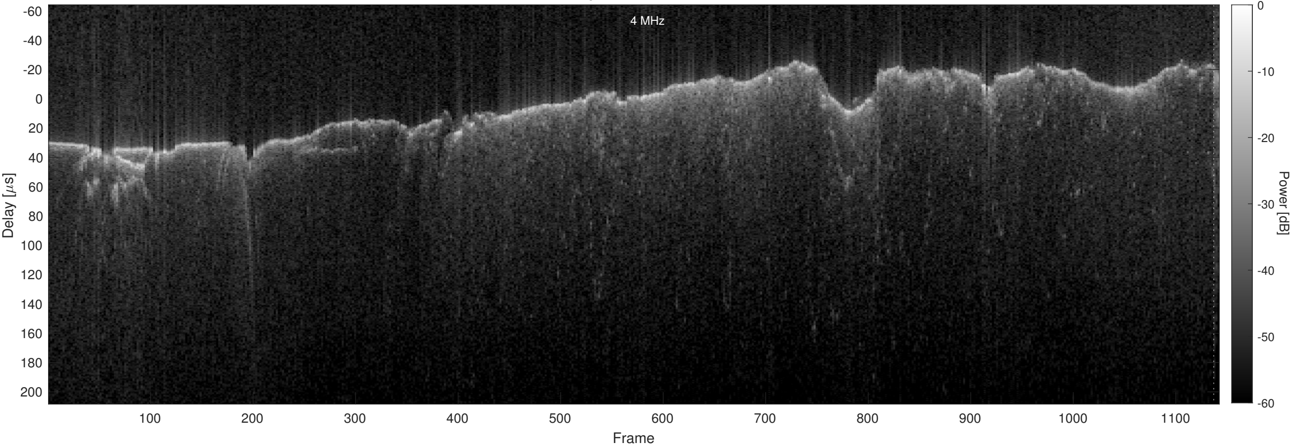
Orbit 15416, Chapman, No Window, Channel 2
