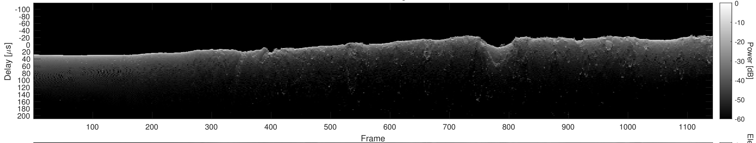
Orbit 15416, Cluttergram
