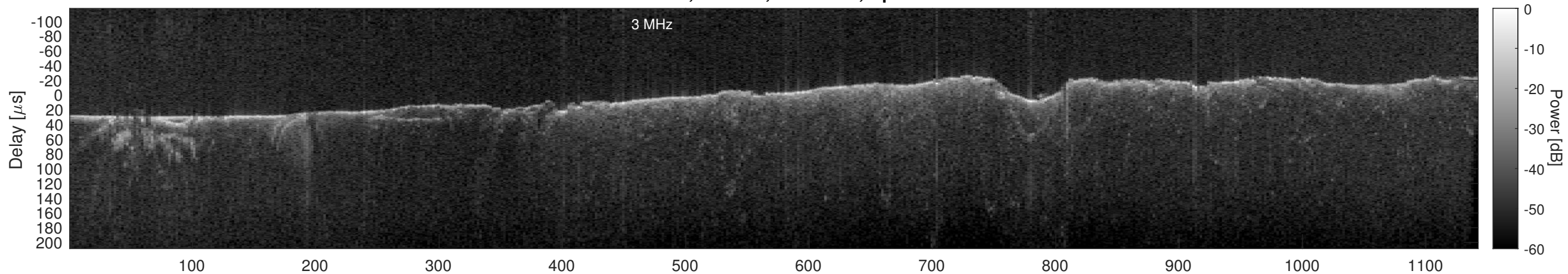
Orbit 15416, Cluttergram
