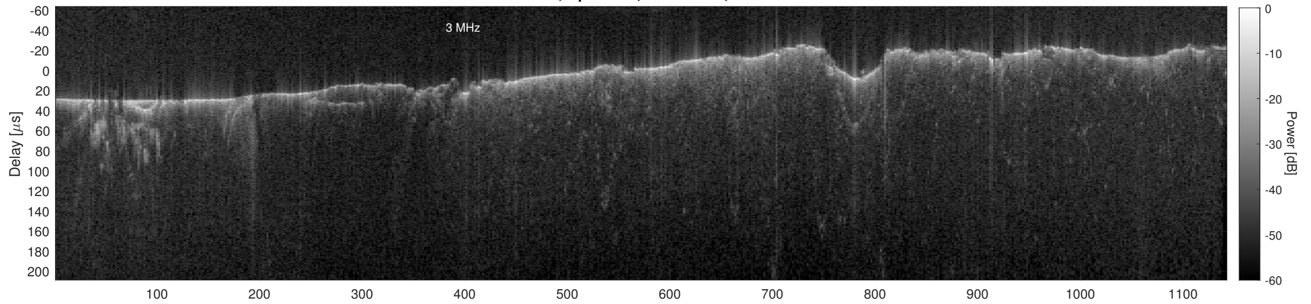
Orbit 15416, Cluttergram
