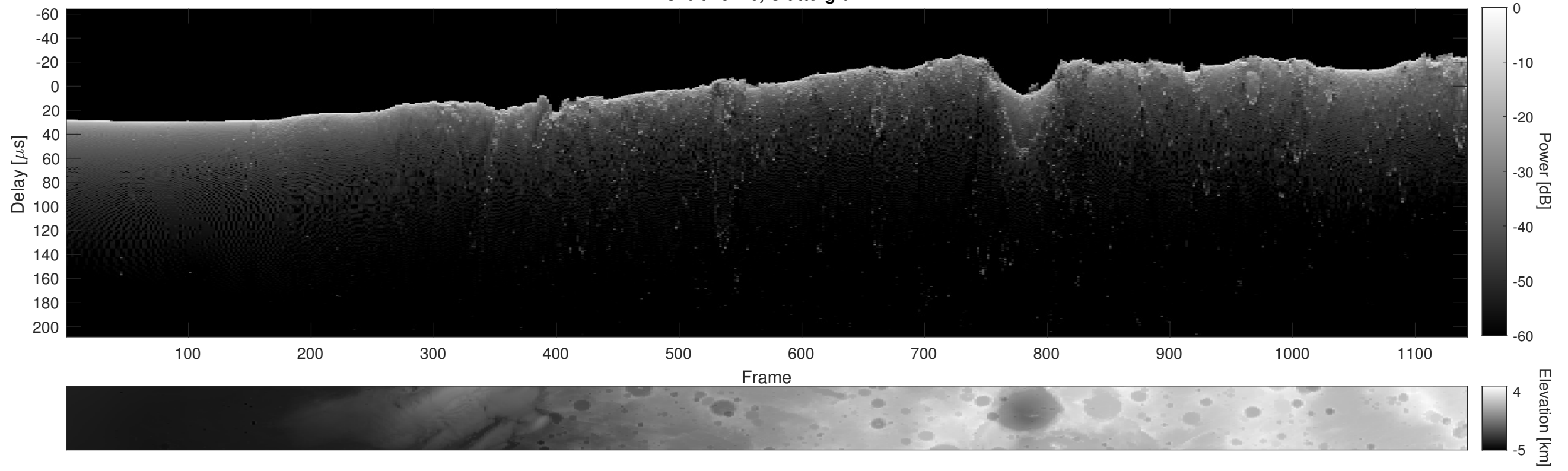
Orbit 15416, Cluttergram
