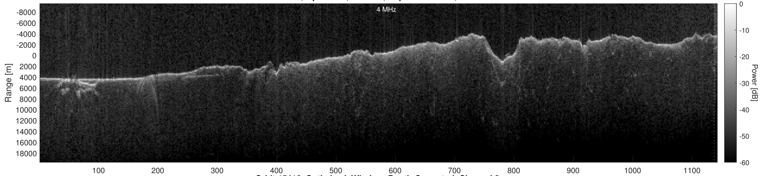
Orbit 15416, Optimized, Window, Depth-Corrected, Channel 2
