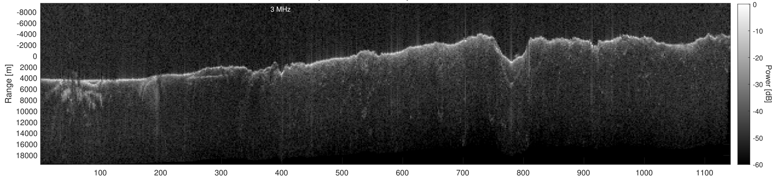
Orbit 15416, Depth-Corrected Cluttergram
