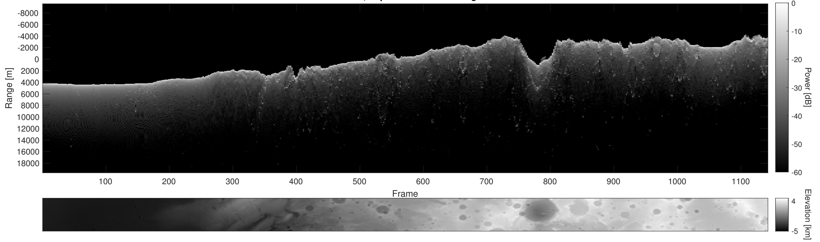
Orbit 15416, Depth-Corrected Cluttergram
