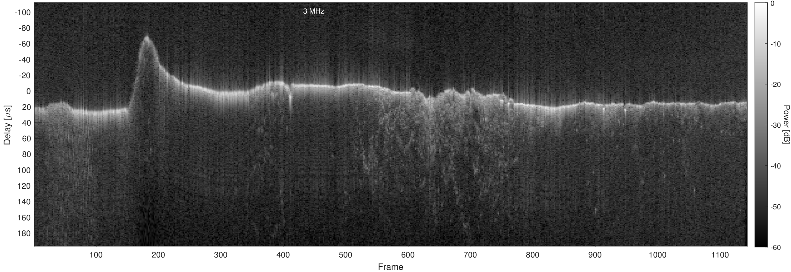
Orbit 15419, Chapman, No Window, Channel 2
