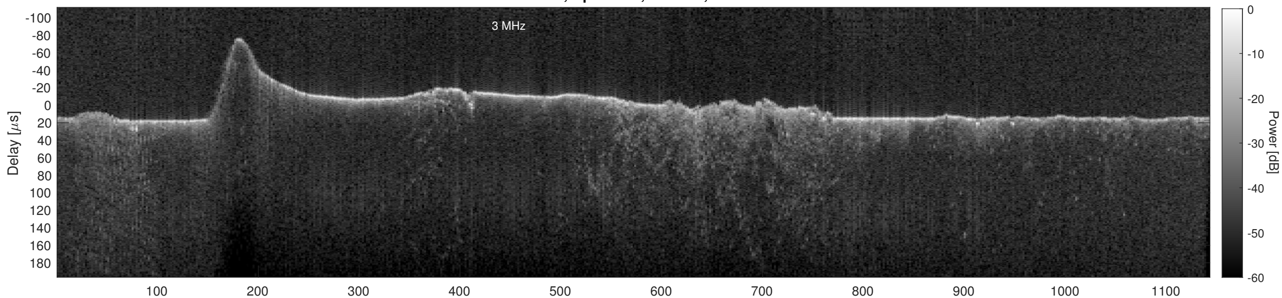
Orbit 15419, Cluttergram
