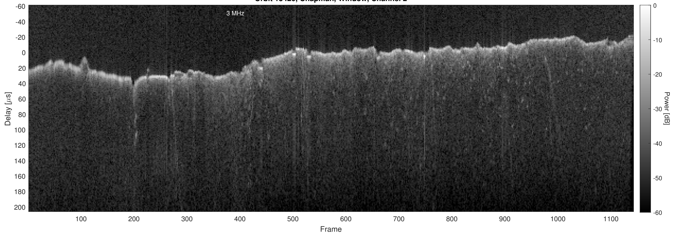
Orbit 15420, Chapman, Window, Channel 2
