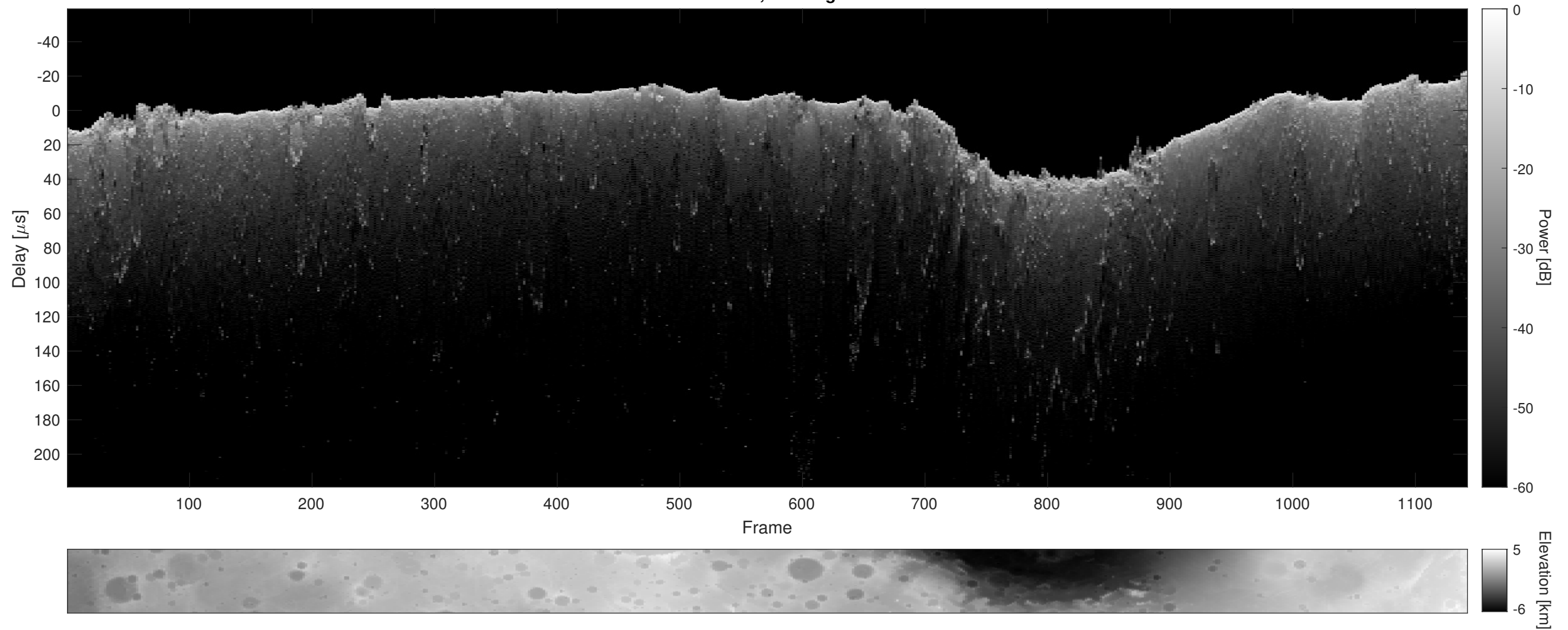
Orbit 15421, Cluttergram
