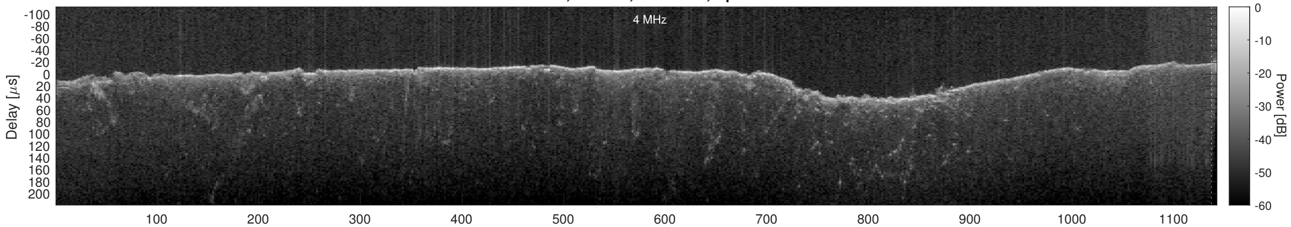
Orbit 15421, Cluttergram
