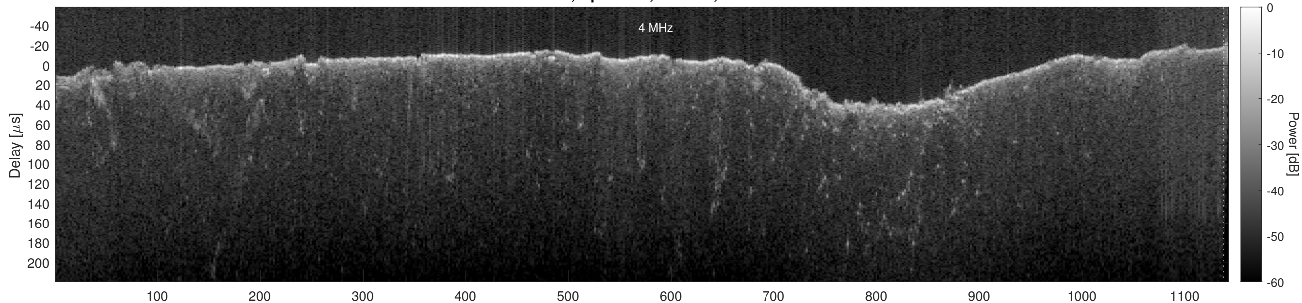
Orbit 15421, Optimized, Window, Channel 2
