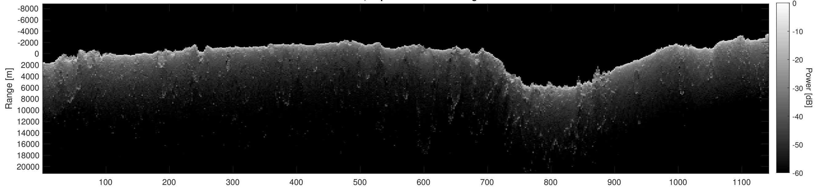
Orbit 15421, Depth-Corrected Cluttergram
