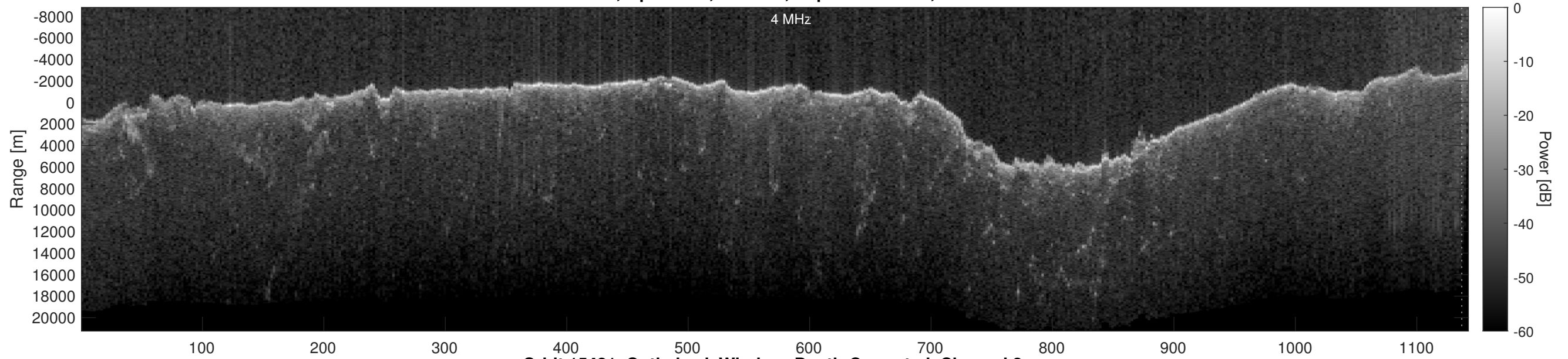
Orbit 15421, Optimized, Window, Depth-Corrected, Channel 2
