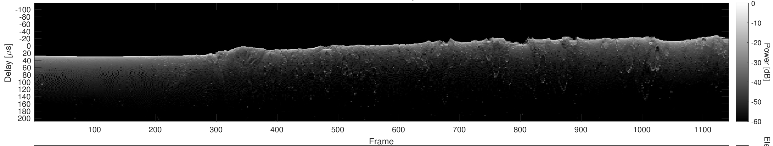
Orbit 15423, Cluttergram
