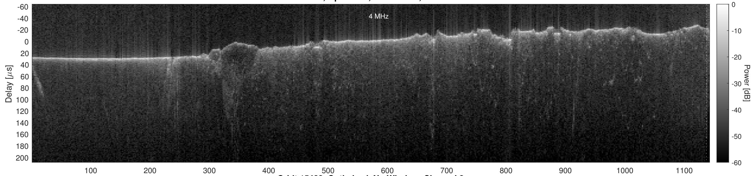
Orbit 15423, Optimized, No Window, Channel 2
