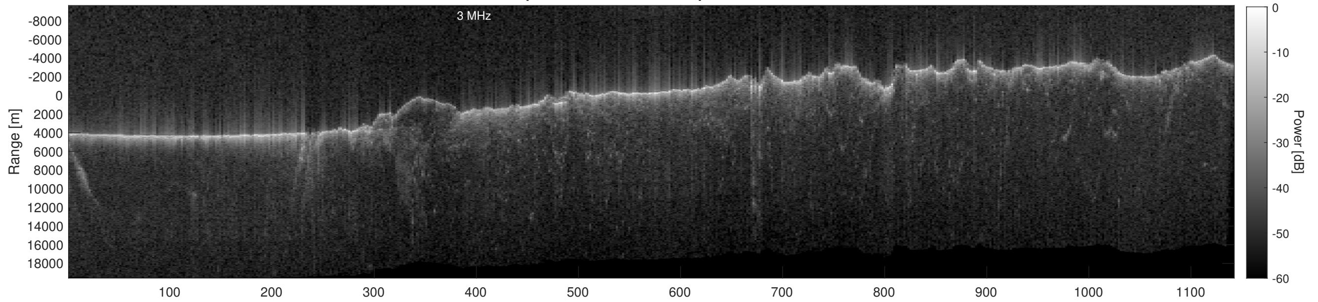
Orbit 15423, Depth-Corrected Cluttergram
