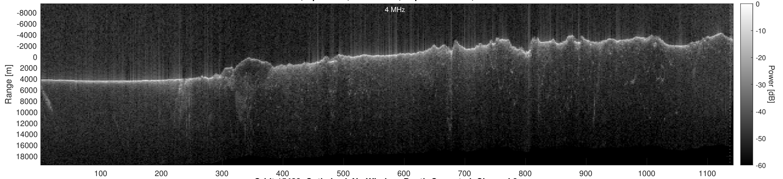
Orbit 15423, Optimized, No Window, Depth-Corrected, Channel 2
