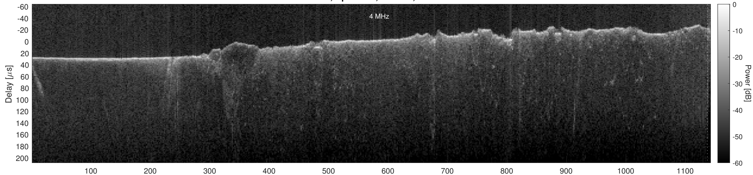
Orbit 15423, Optimized, Window, Channel 2
