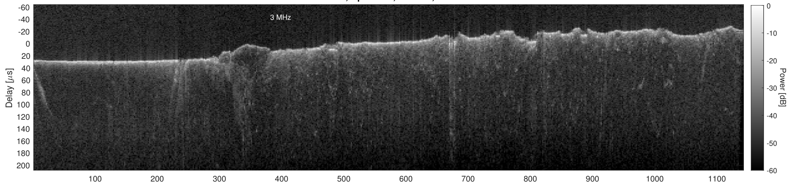
Orbit 15423, Cluttergram
