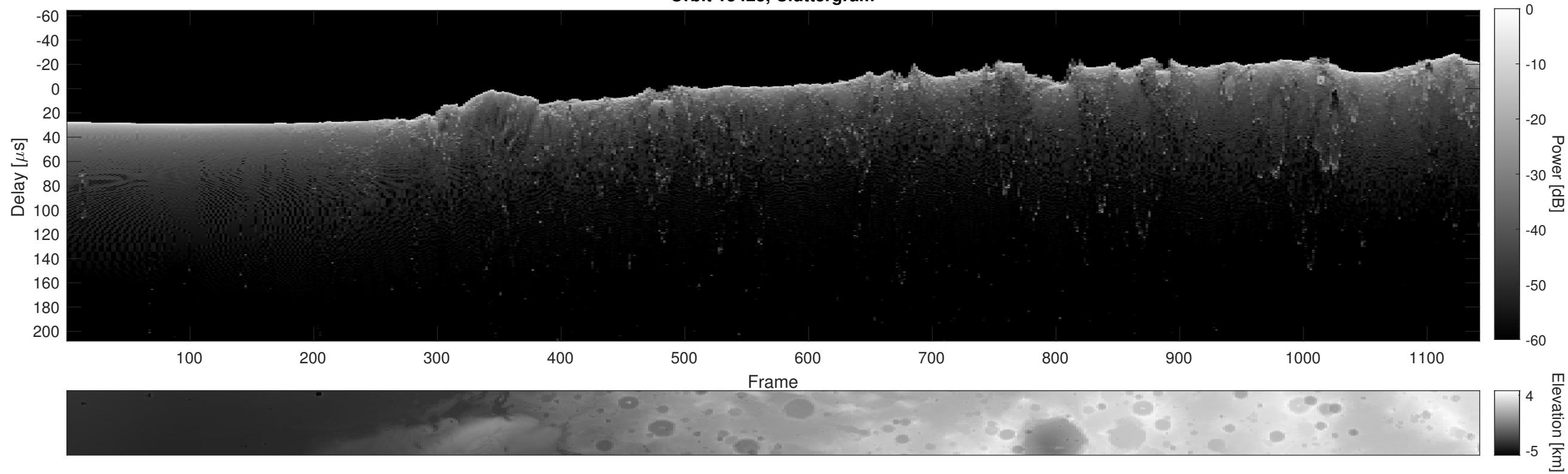
Orbit 15423, Cluttergram
