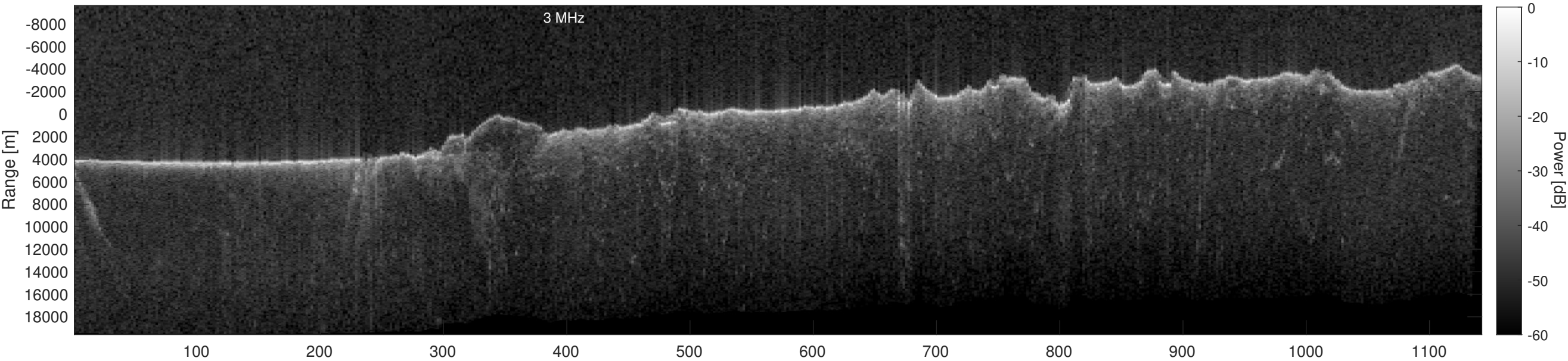
Orbit 15423, Depth-Corrected Cluttergram
