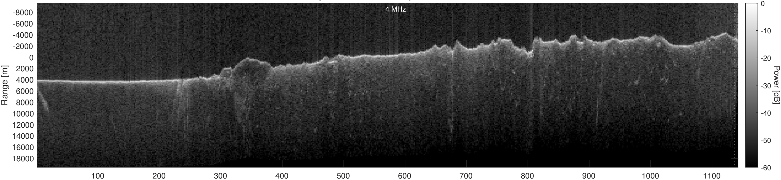
Orbit 15423, Optimized, Window, Depth-Corrected, Channel 2
