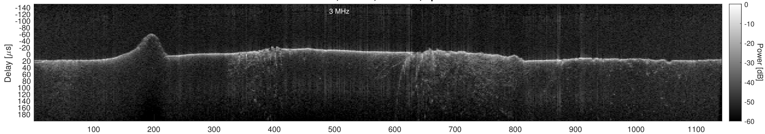
Orbit 15426, Cluttergram
