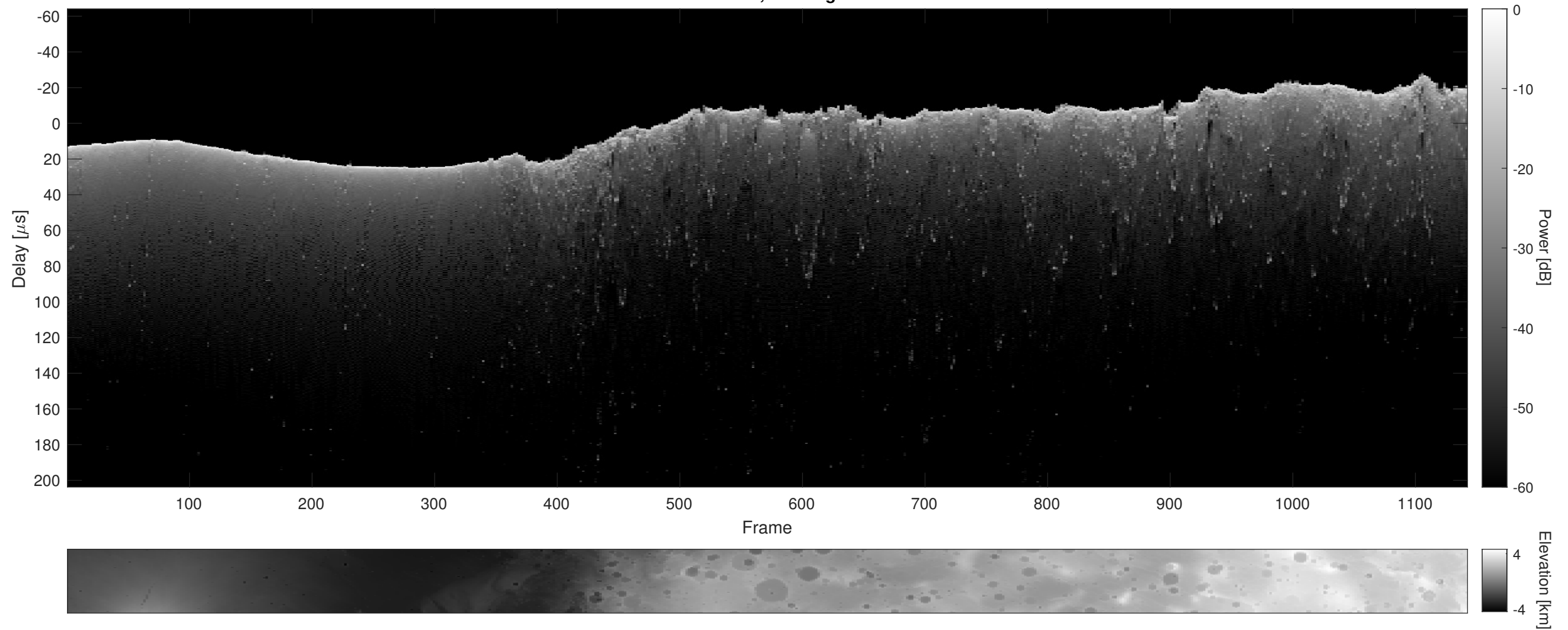
Orbit 15427, Cluttergram
