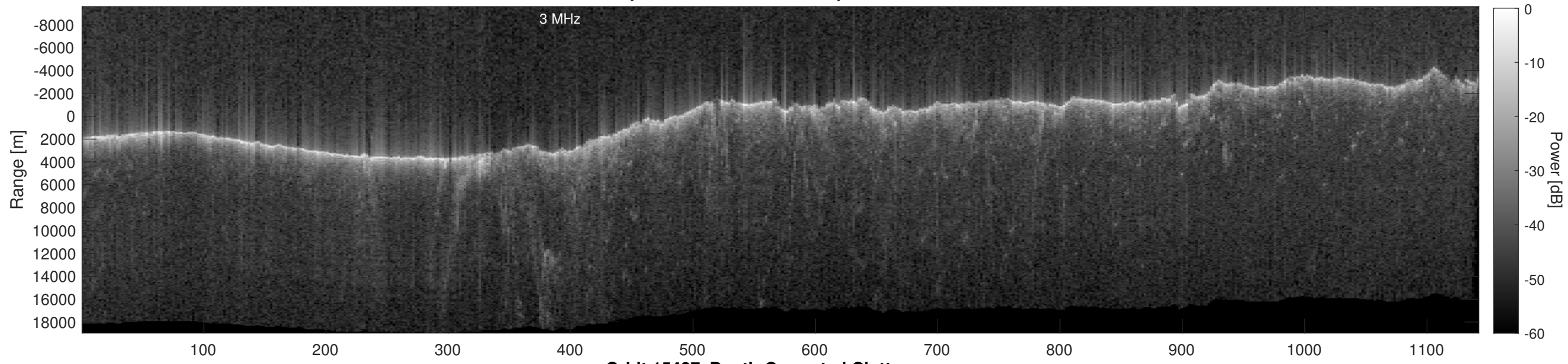
Orbit 15427, Depth-Corrected Cluttergram
