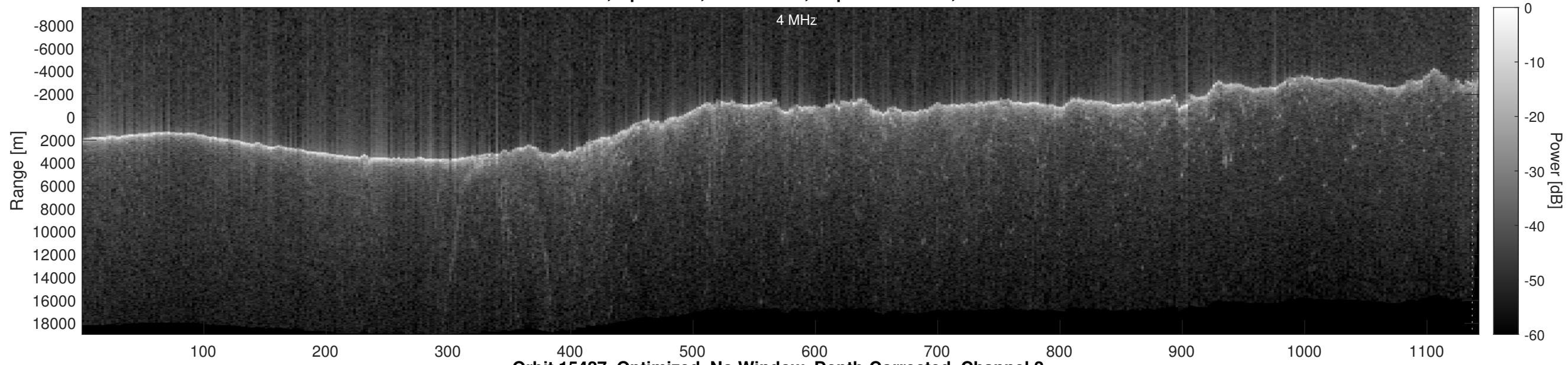
Orbit 15427, Optimized, No Window, Depth-Corrected, Channel 2
