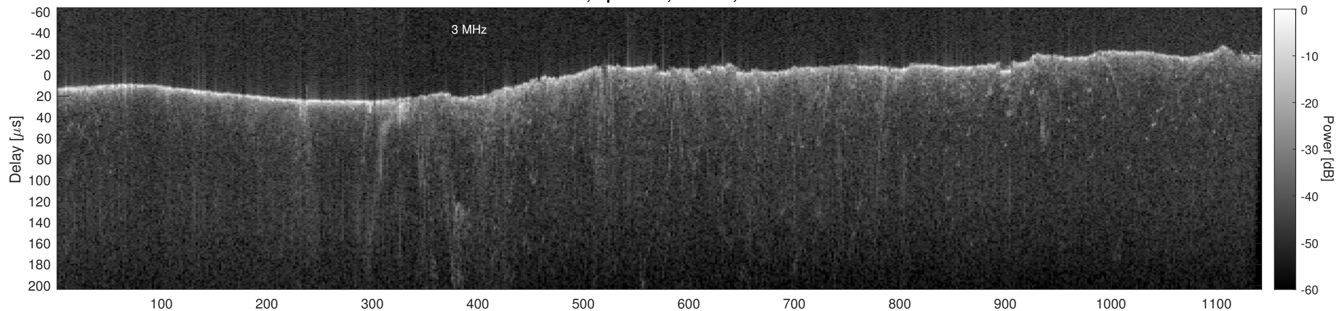
Orbit 15427, Cluttergram
