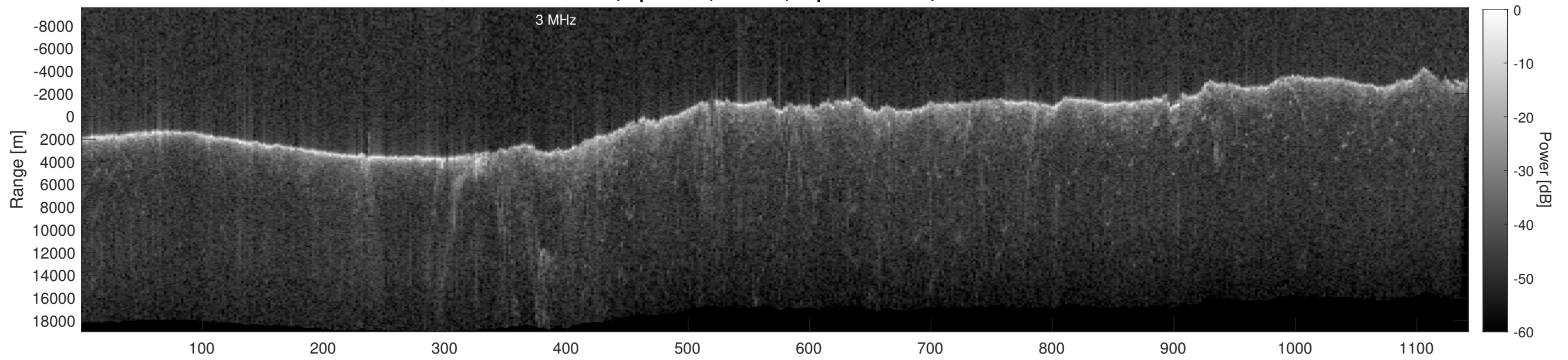
Orbit 15427, Depth-Corrected Cluttergram
