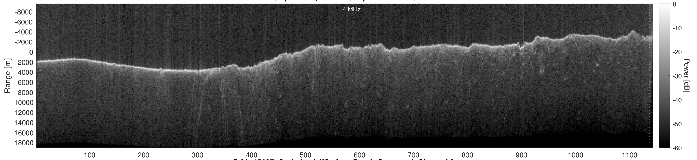
Orbit 15427, Optimized, Window, Depth-Corrected, Channel 2
