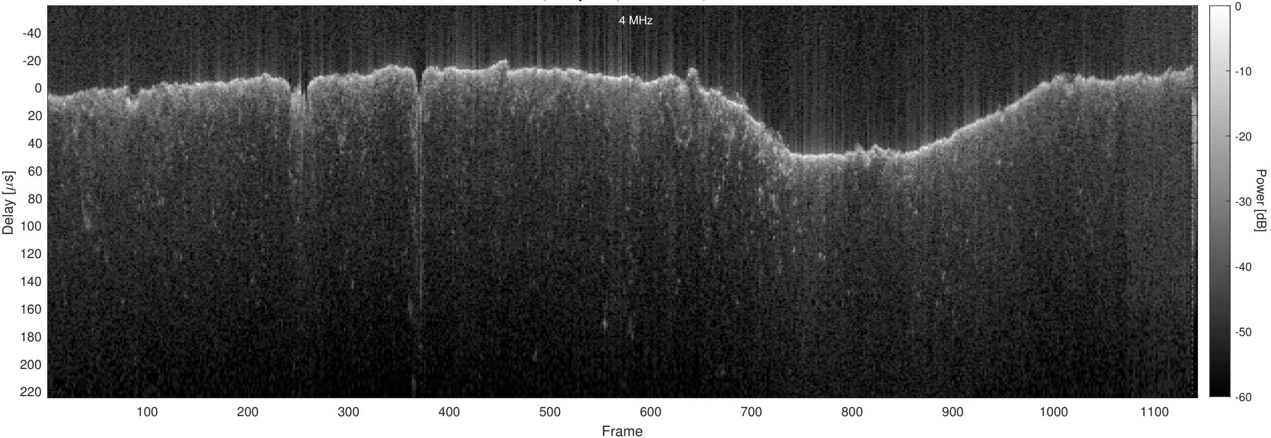
Orbit 15428, Chapman, No Window, Channel 2
