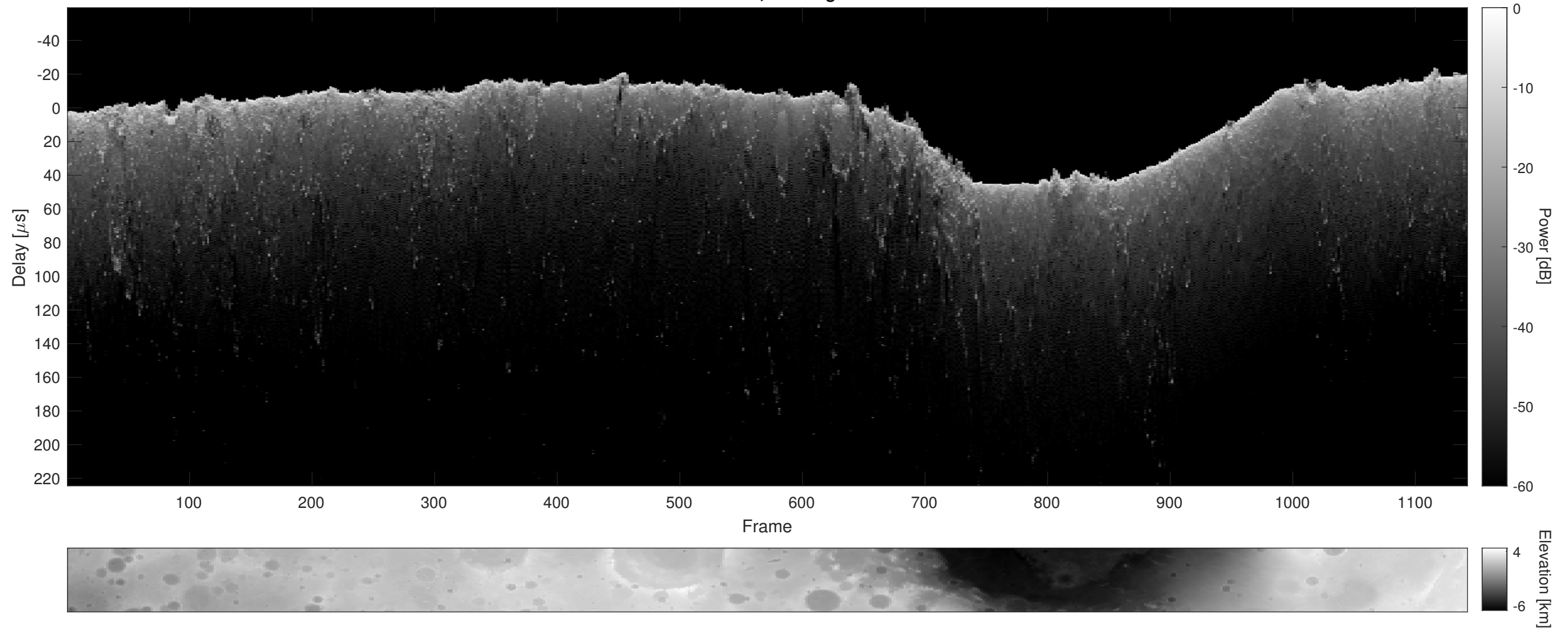
Orbit 15428, Cluttergram
